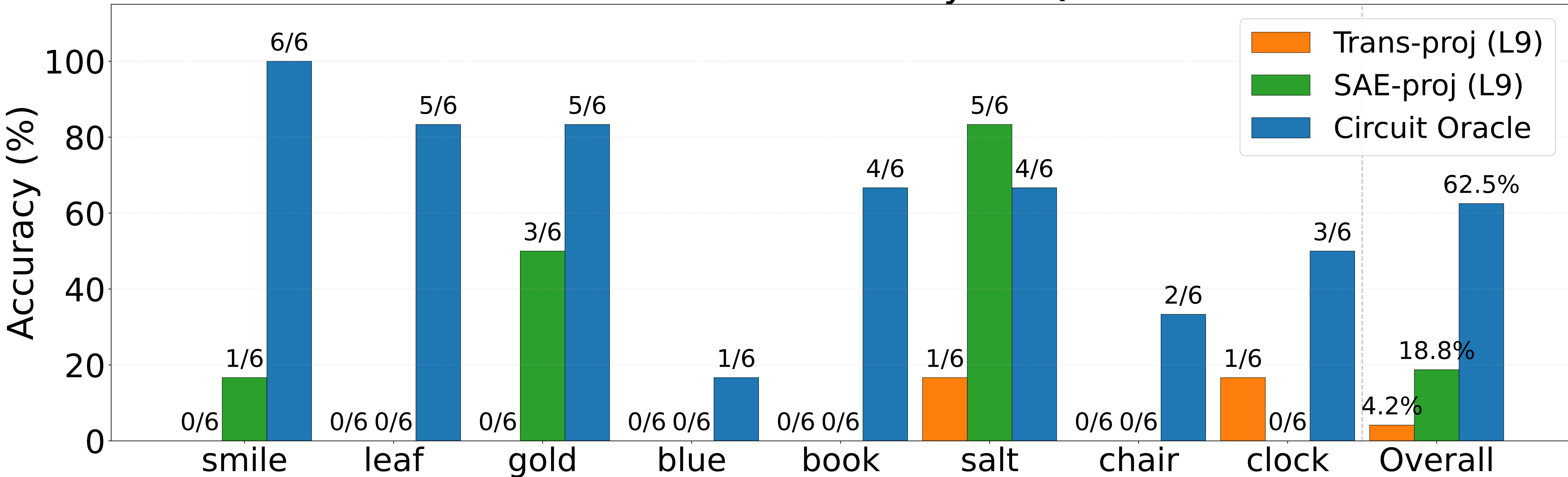
Closed-mode secret elicitation accuracy on Qwen3-8B taboo LoRAs
