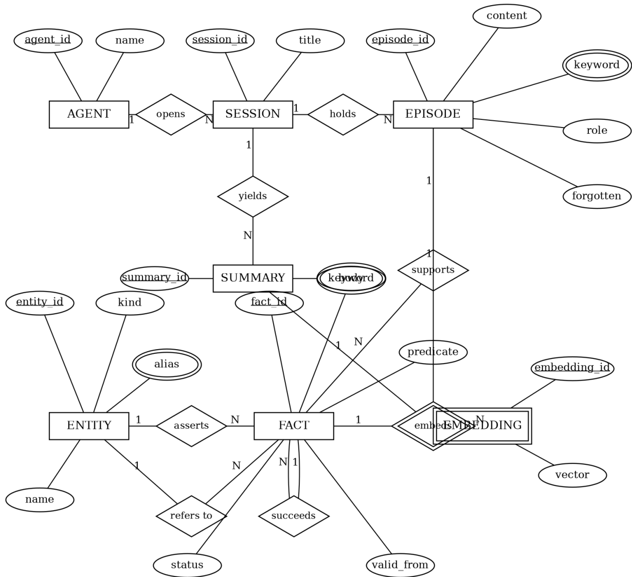
Figure 2: ER diagram of the memory store.
