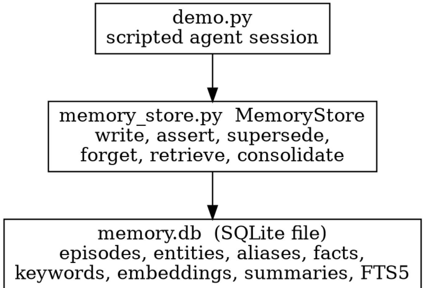
Figure 1. How the pieces fit. demo.py calls MemoryStore , and that module is the only writer of memory.db .
