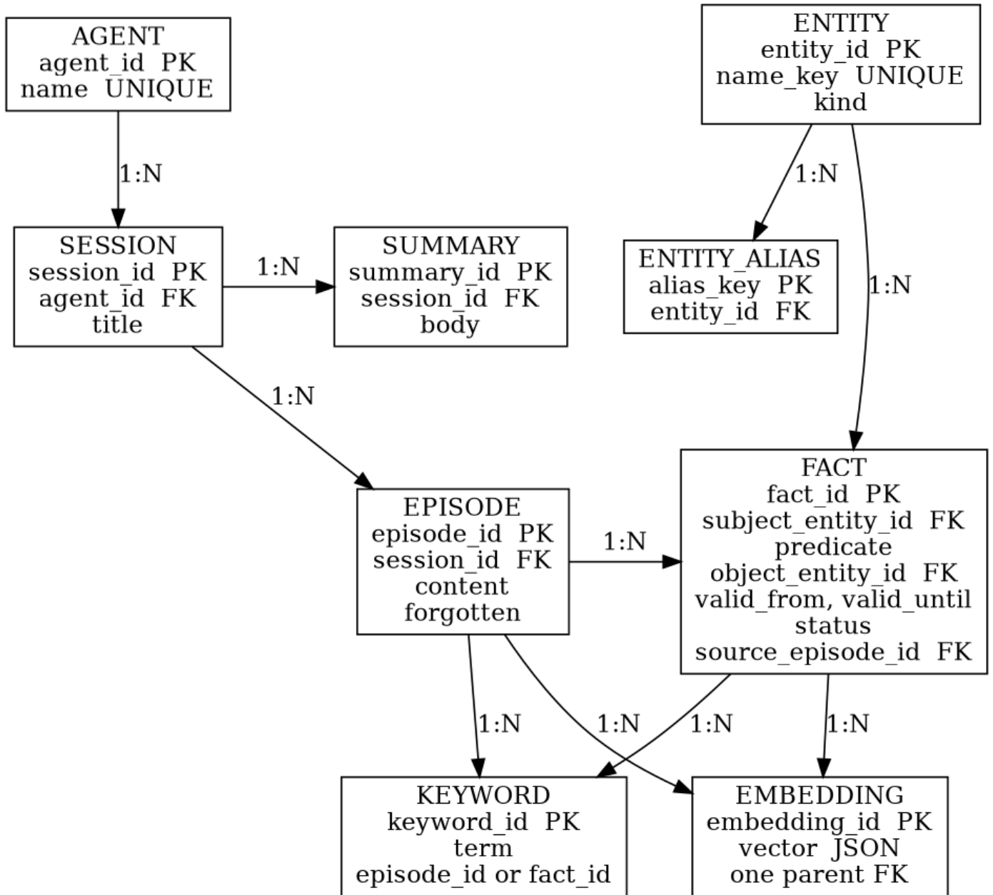
Figure 2. The tables and the main relationships. Edges are marked 1:N. Drawn with Graphviz, default boxes.
