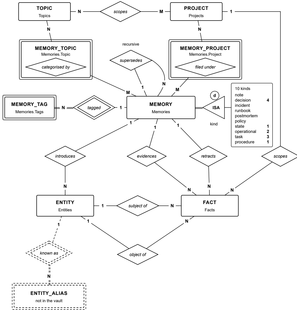
Figure 2 — Entity-relationship diagram, Chen notation
