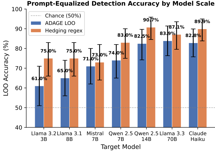
Figure 2: Prompt-equalized detection accuracy by model scale (LOO pipeline in blue, hedging regex in orange). Error bars are bootstrap 95% CIs. Models \leq 7\text{B} cluster at 61–74% and models \geq 14\text{B} at 82.5–84% (pooled p < 0.0001 , exploratory post-hoc comparison, not pre-registered); no individual adjacent increment is significant after joint Holm-Bonferroni correction.
