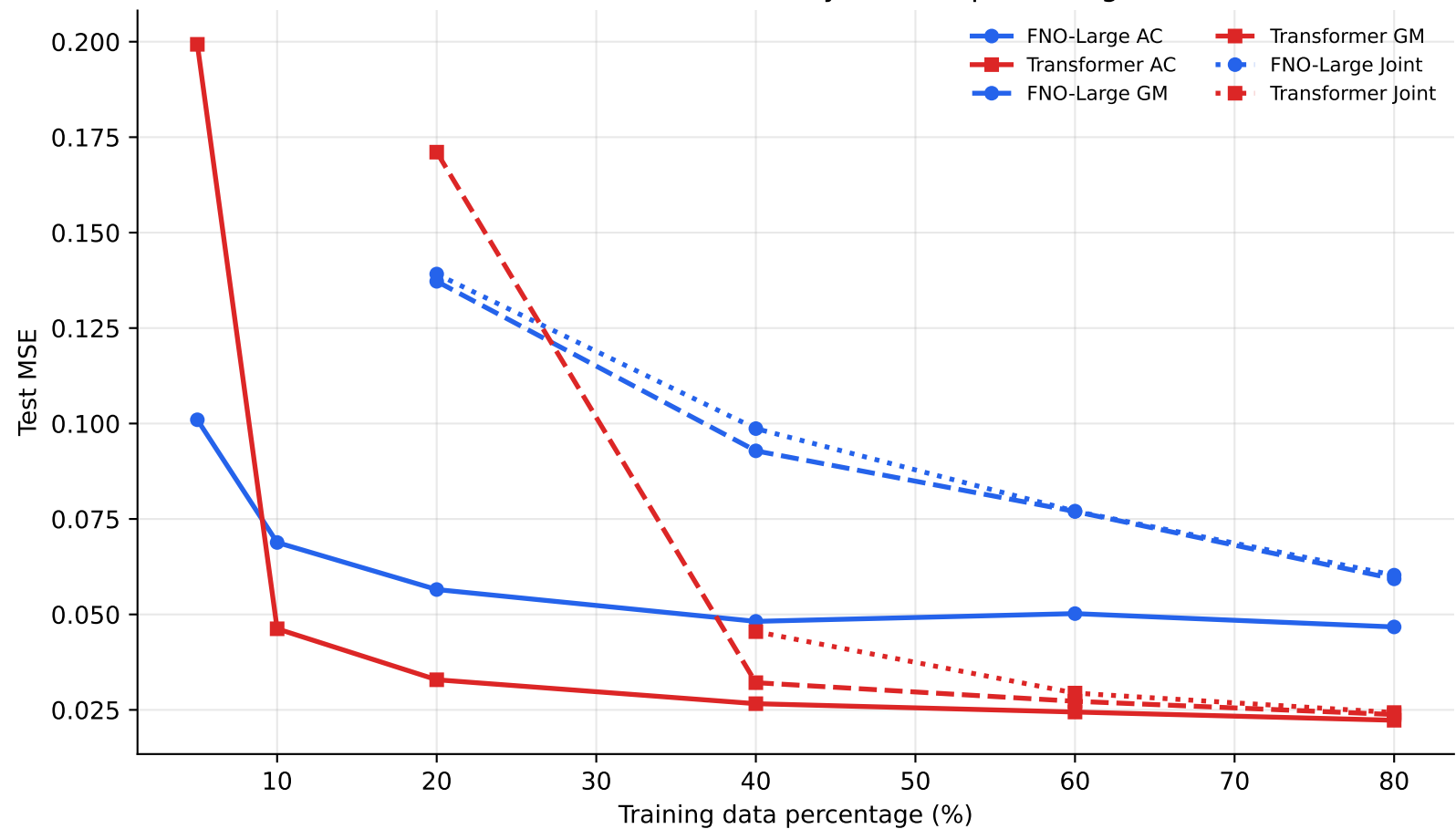
F6 18m O2 data efficiency: MSE vs percentage
