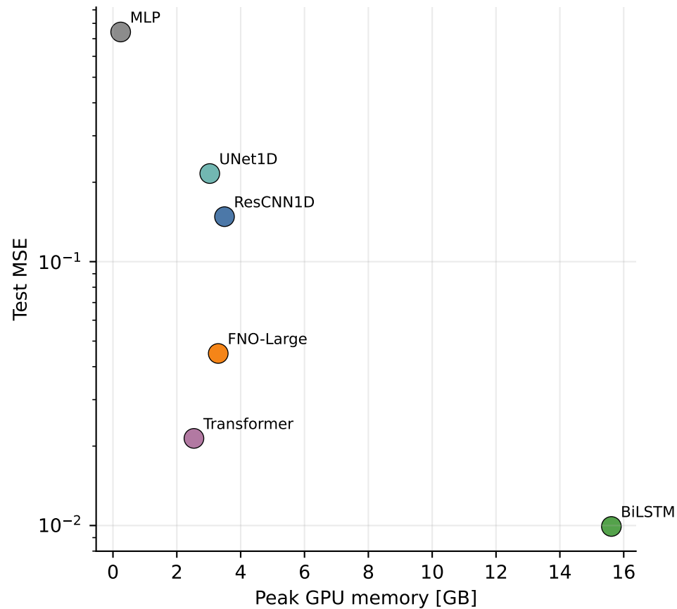
O1 Test MSE vs Resource Tradeoffs
