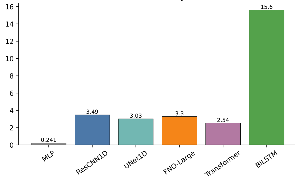
Test inference latency [ms/sample]
