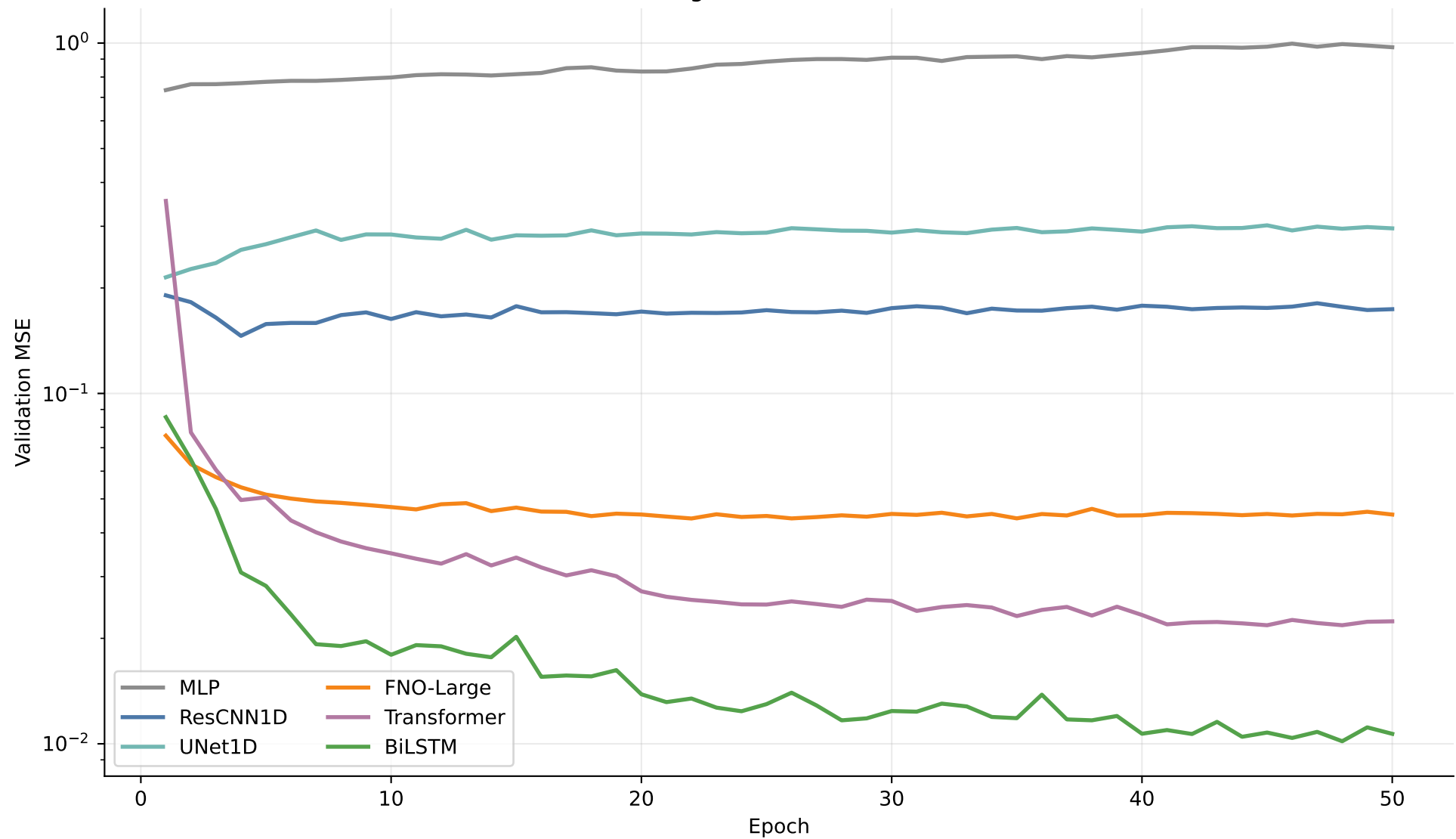
O1 Training Curves: Validation MSE
