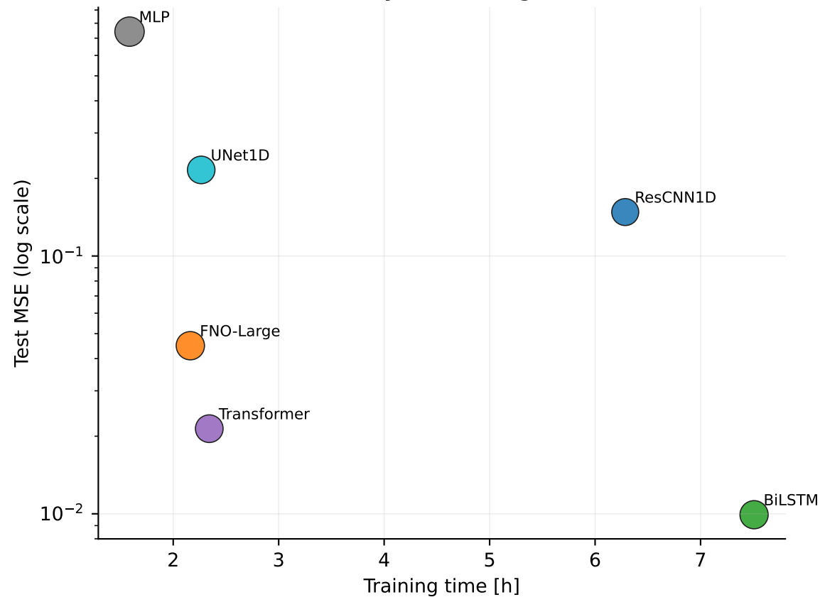
Accuracy vs Training Cost
