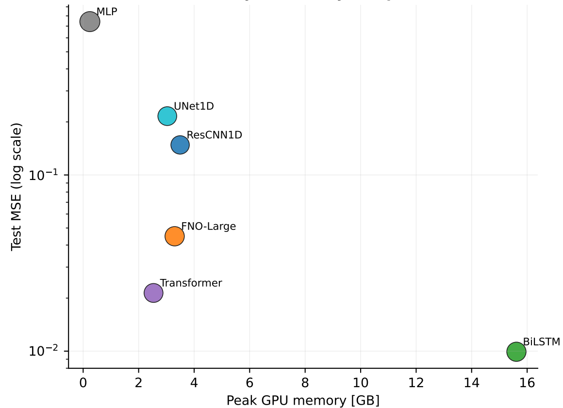
Accuracy vs Memory Footprint
