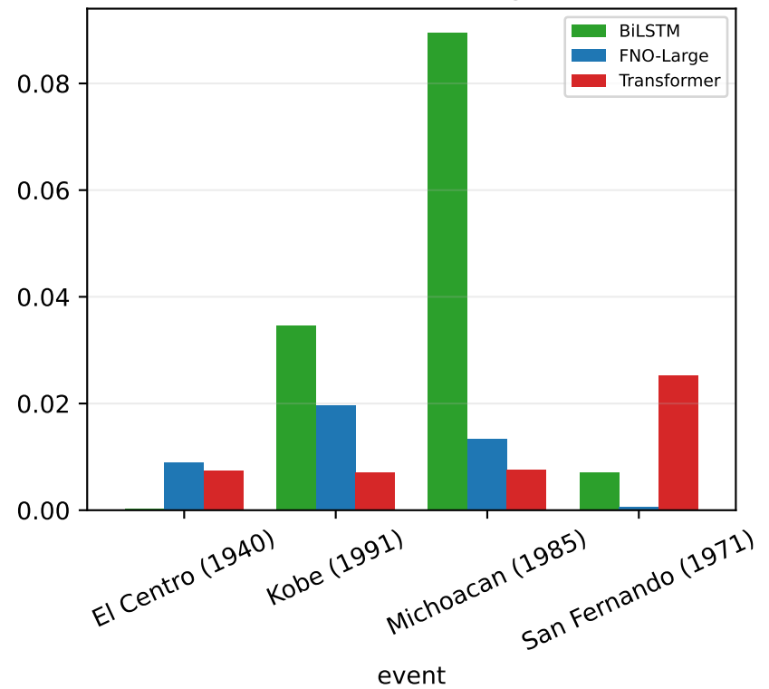
PFA abs. error [g]
