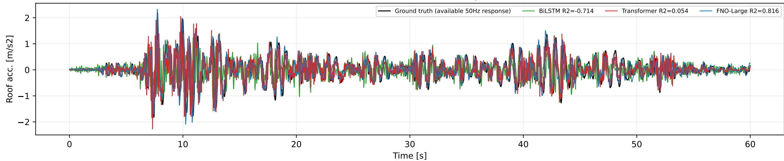
Kobe (1991): native GM 100Hz, response GT 50Hz
