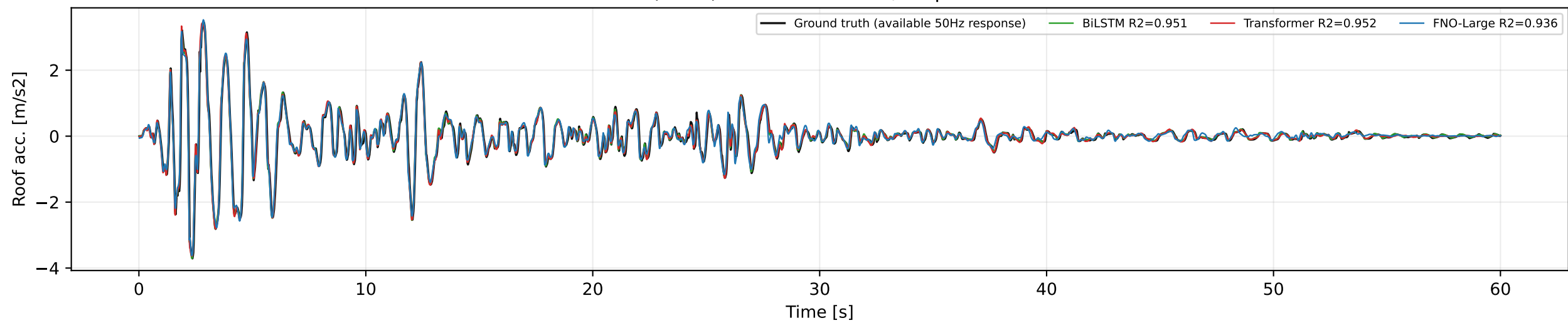
San Fernando (1971): native GM 50Hz, response GT 50Hz
