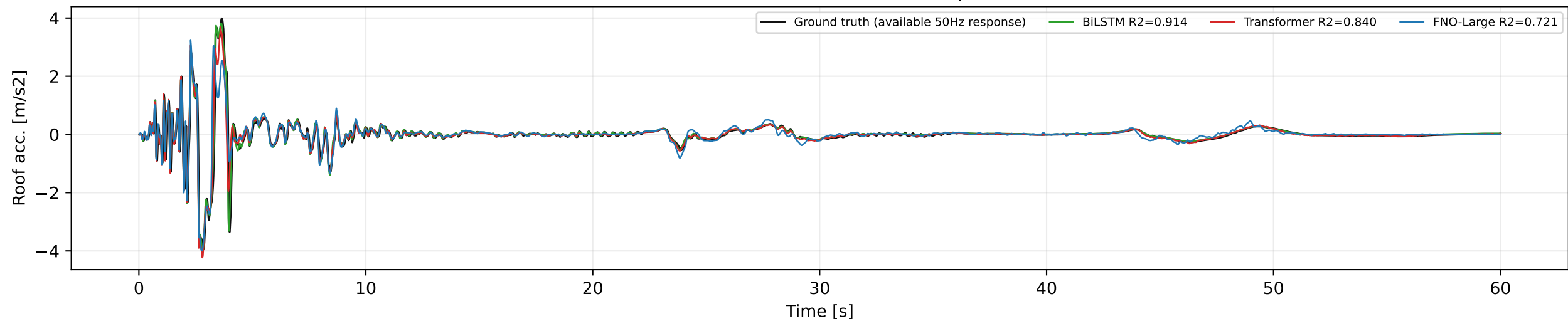
Michoacan (1985): native GM 200Hz, response GT 50Hz
