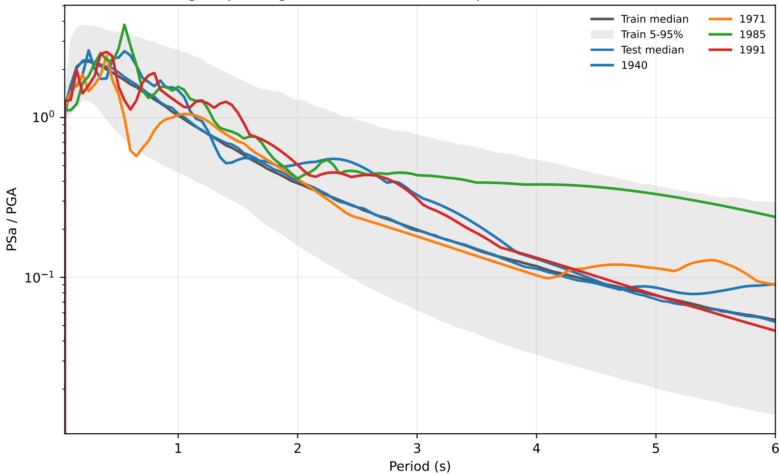
Nigam-Jennings Pseudo-Acceleration Spectra (PGA-normalized)
