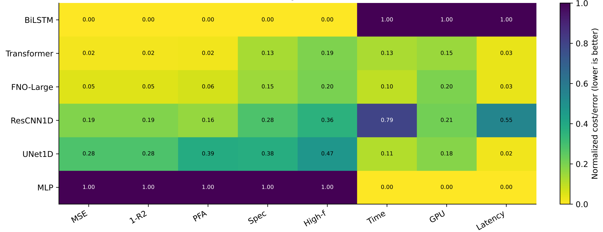
Normalized Accuracy and Resource Profile
