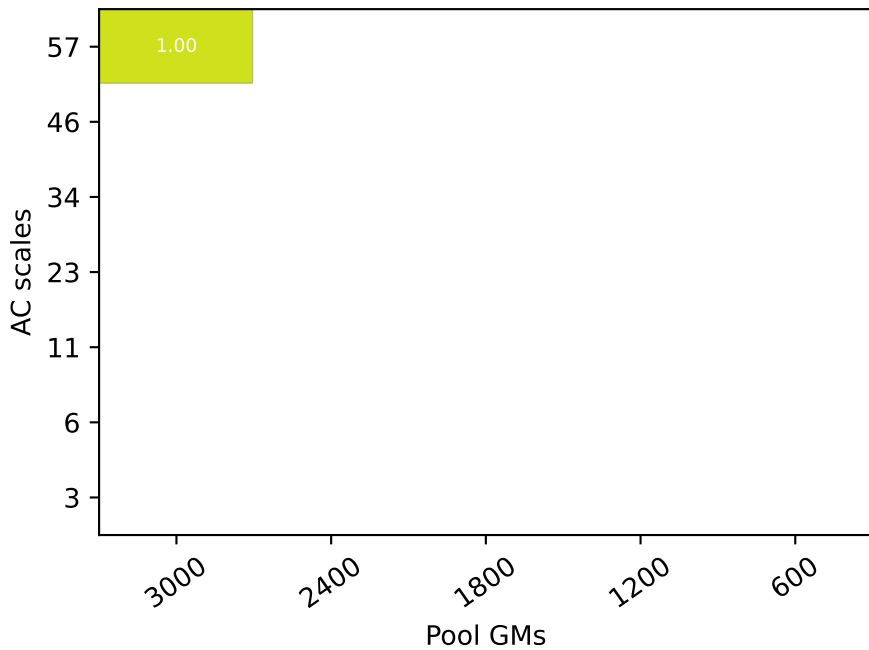
FNO-Large
