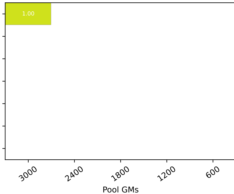
Transformer
