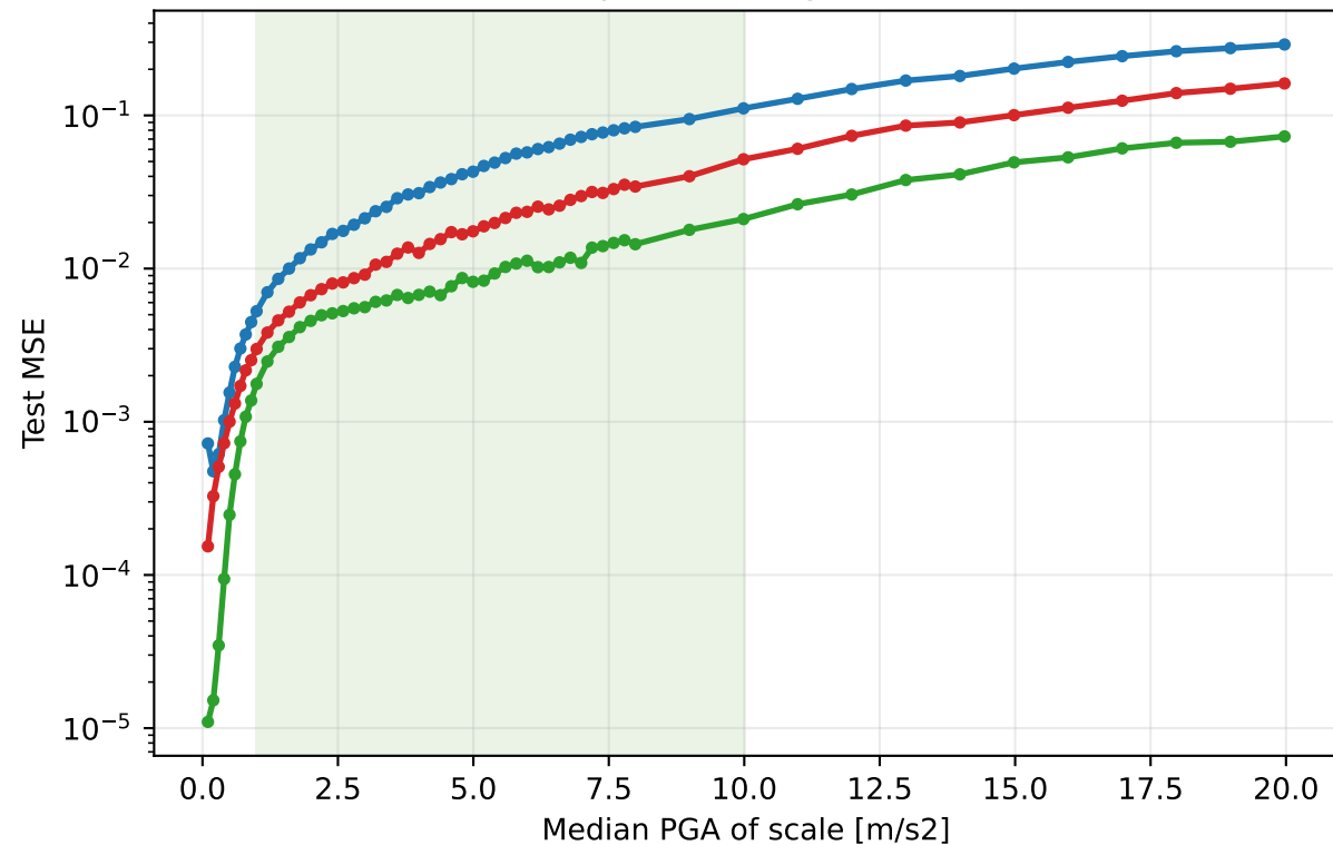
PGA extrapolation degradation: MSE
