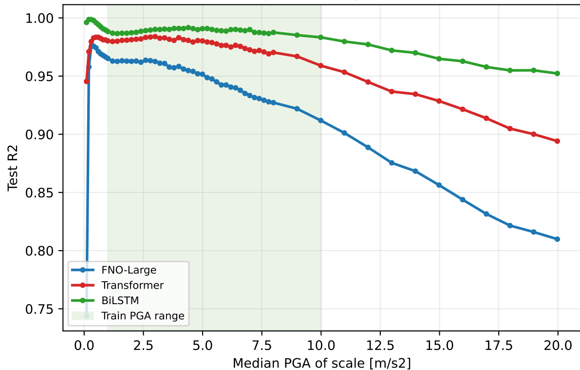
PGA extrapolation degradation: R2
