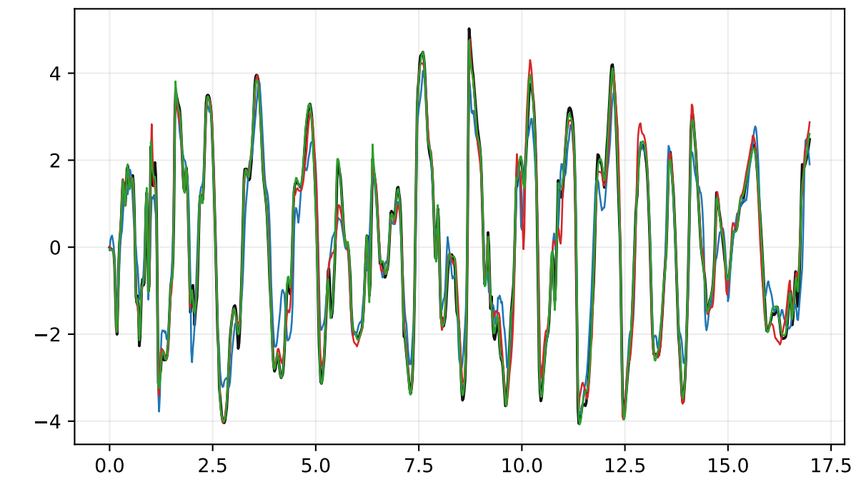
GM 3393 / scale 56
