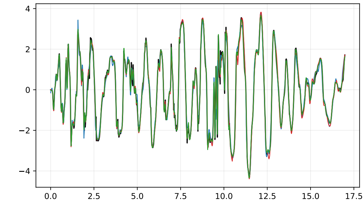
GM 3393 / scale 46
