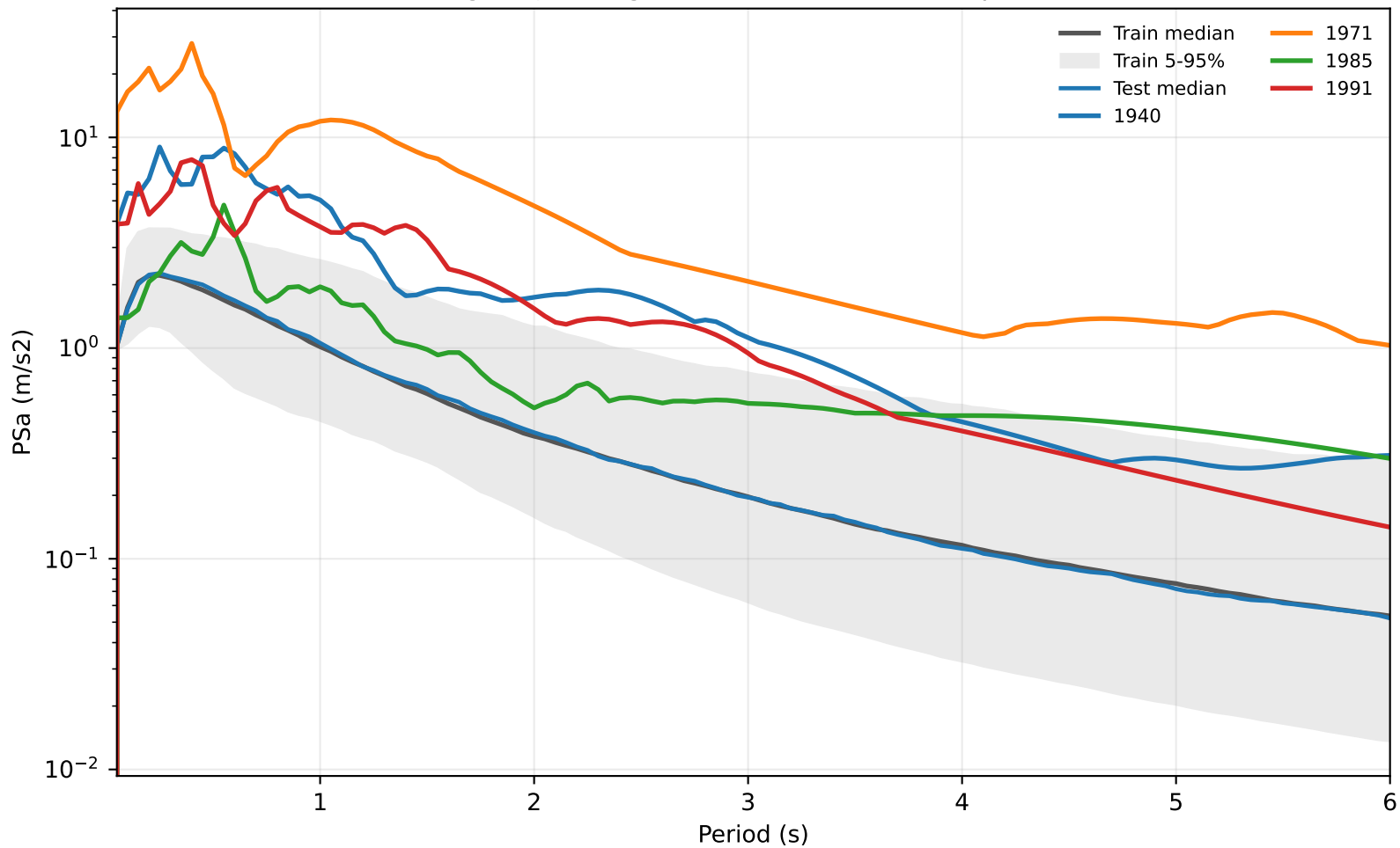
Nigam-Jennings Pseudo-Acceleration Spectra
