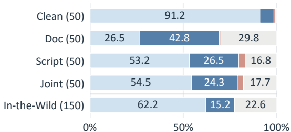
(a) Raw Package → +AST
