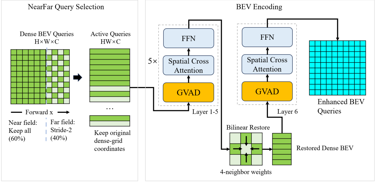
Figure 5: Overall architecture of the GeoVis-BEV encoder. Three forward-facing images are processed by ResNet-FPN and fed to a six-layer encoder. GVAD updates BEV tokens in every layer. NearFar retains dense near-field queries and regularly sparsely samples far-field queries in the first five layers; after restoration to a dense grid, the final layer performs image-conditioned refinement.
