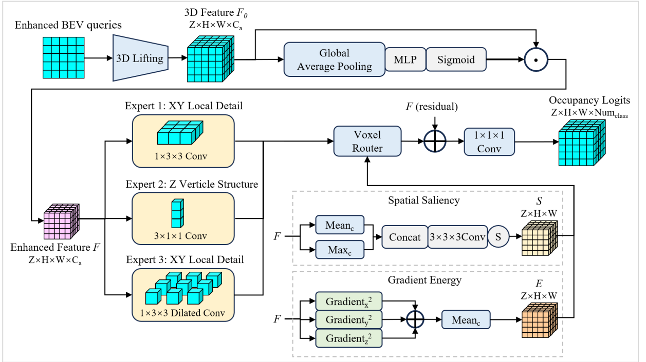
Figure 7: Agri-AMoE 3D occupancy decoder. 2D BEV tokens are lifted into a 3D volume and enhanced by channel attention. Enhanced features are passed in parallel to three anisotropic experts and used to compute spatial saliency and three-direction gradient energy for per-voxel routing weights. The weighted expert outputs are summed, residually fused, and classified.
