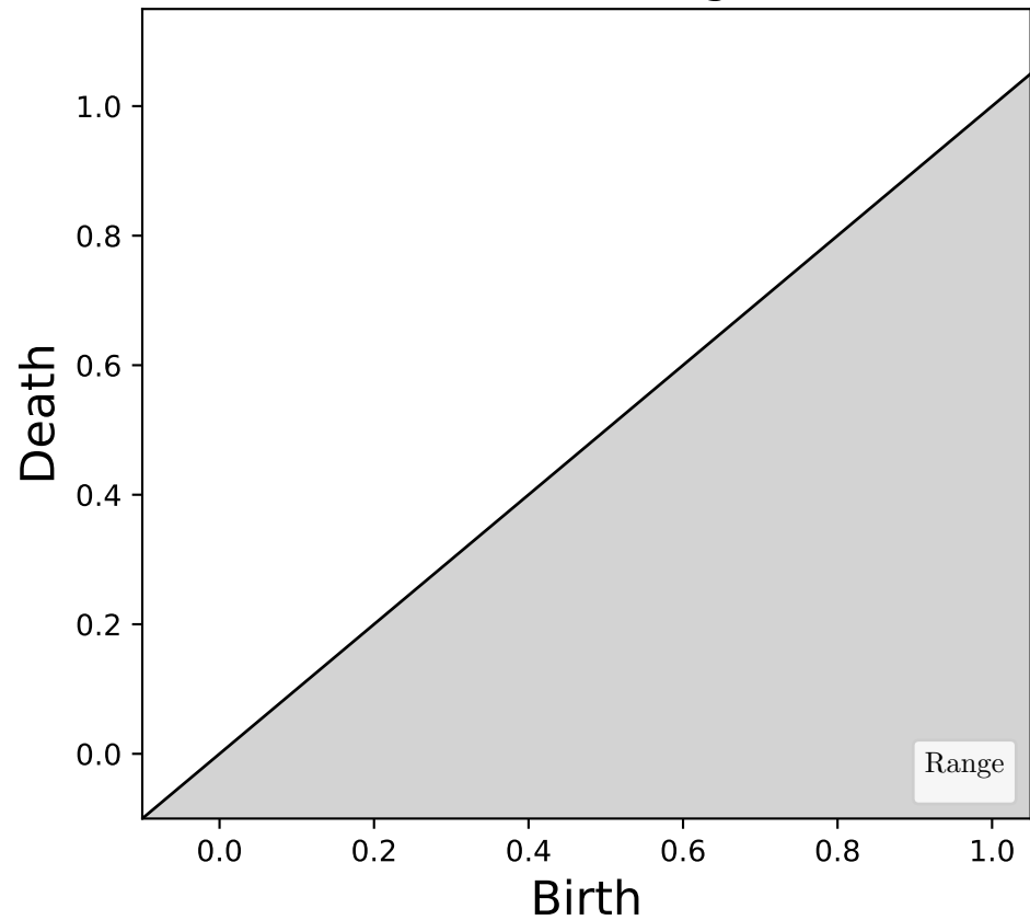
Persistence diagram
