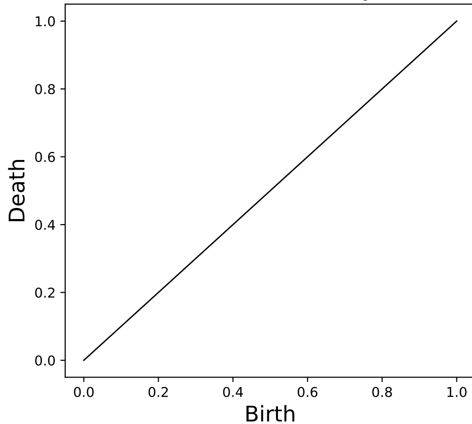
Persistence density
