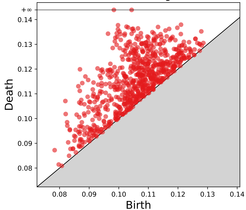
Persistence diagram
