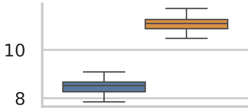
CPU avg (%)
