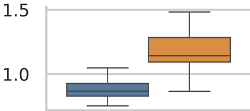
CPU avg (%)
