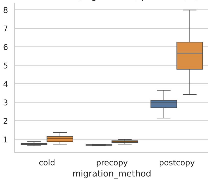
Destination (edge-node-2) | CPU util (%)
