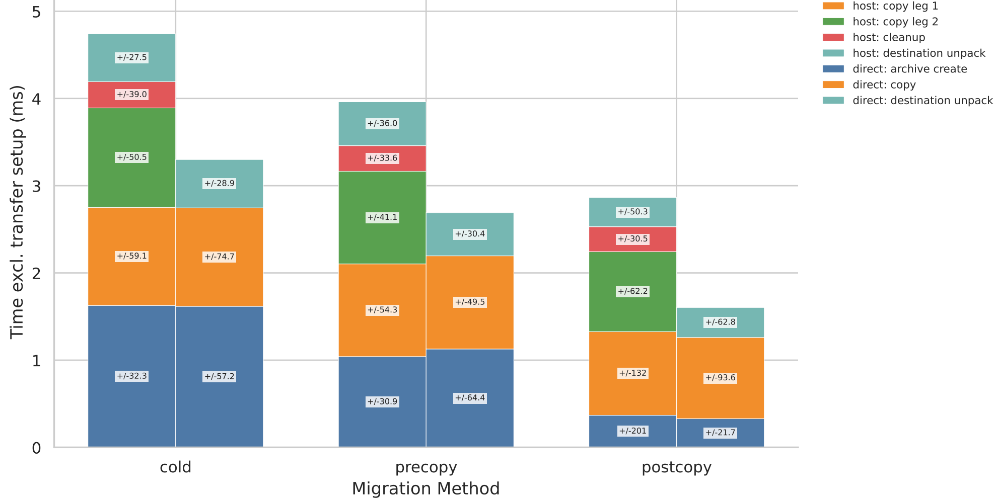
Transfer Phase Breakdown (Mean, setup excluded) - 1 WiFi 6
