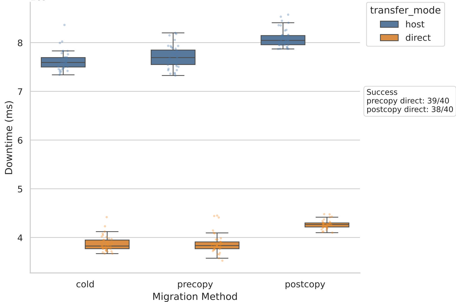
1e3 Migration Downtime by Strategy (Host vs Direct) - 1 WiFi 6
