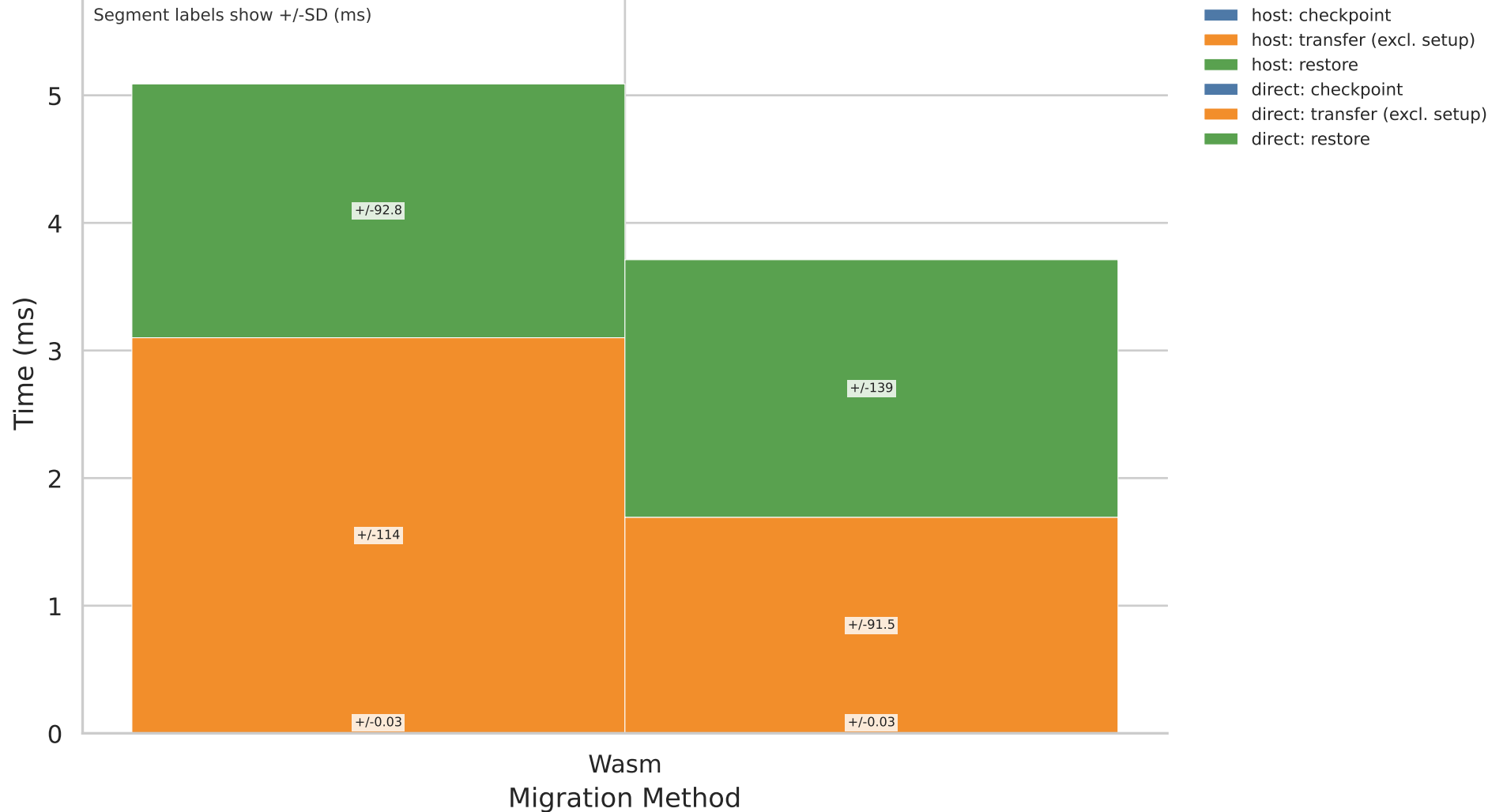
Migration Phase Breakdown (Mean) - 2 5G
