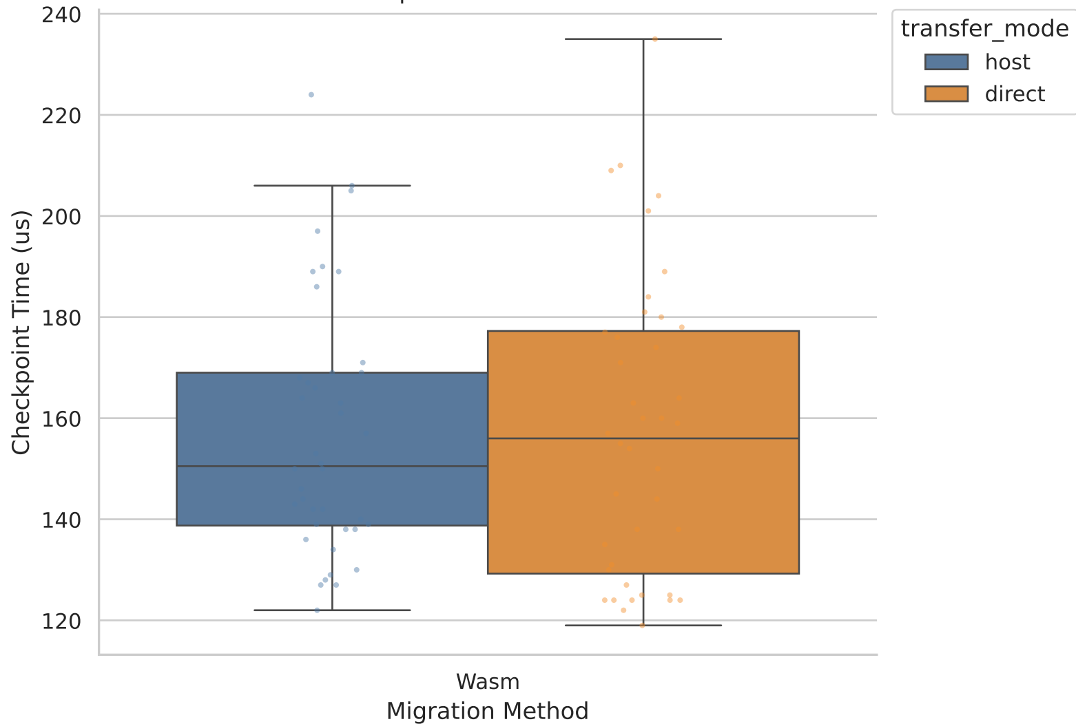
Checkpoint Duration - 3 Lte
