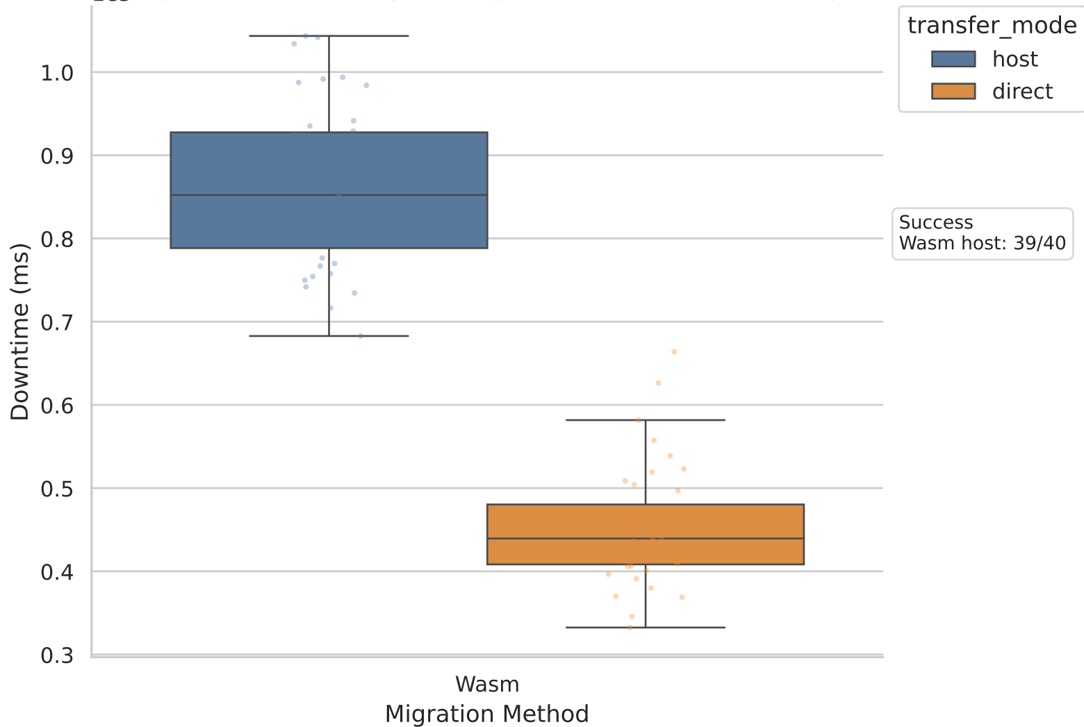
1e5 Migration Downtime by Strategy (Host vs Direct) - 6 TEE Avg
