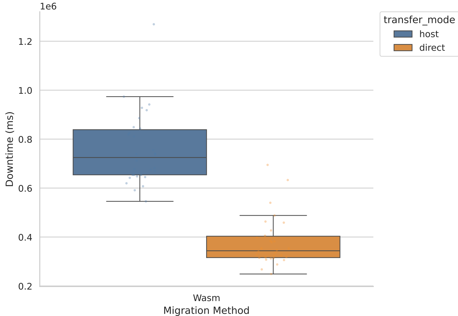
Migration Downtime by Strategy (Host vs Direct) - 7 TEE Worst
