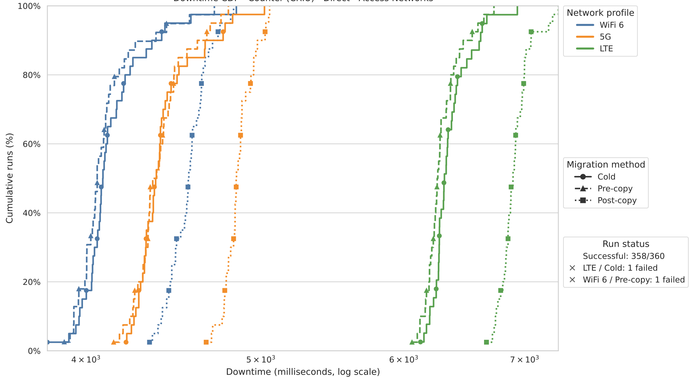
Downtime CDF - Counter (CRIU) - Direct - Access Networks
