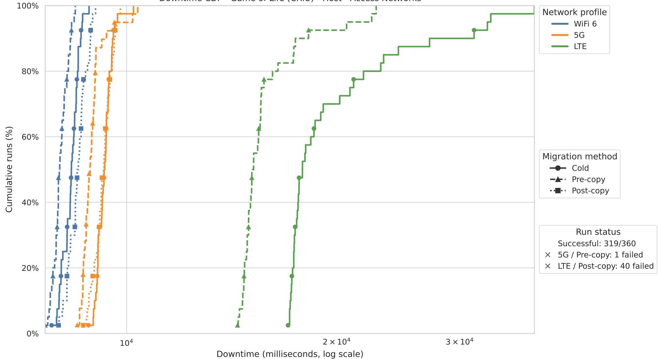
Downtime CDF - Game of Life (CRIU) - Host - Access Networks
