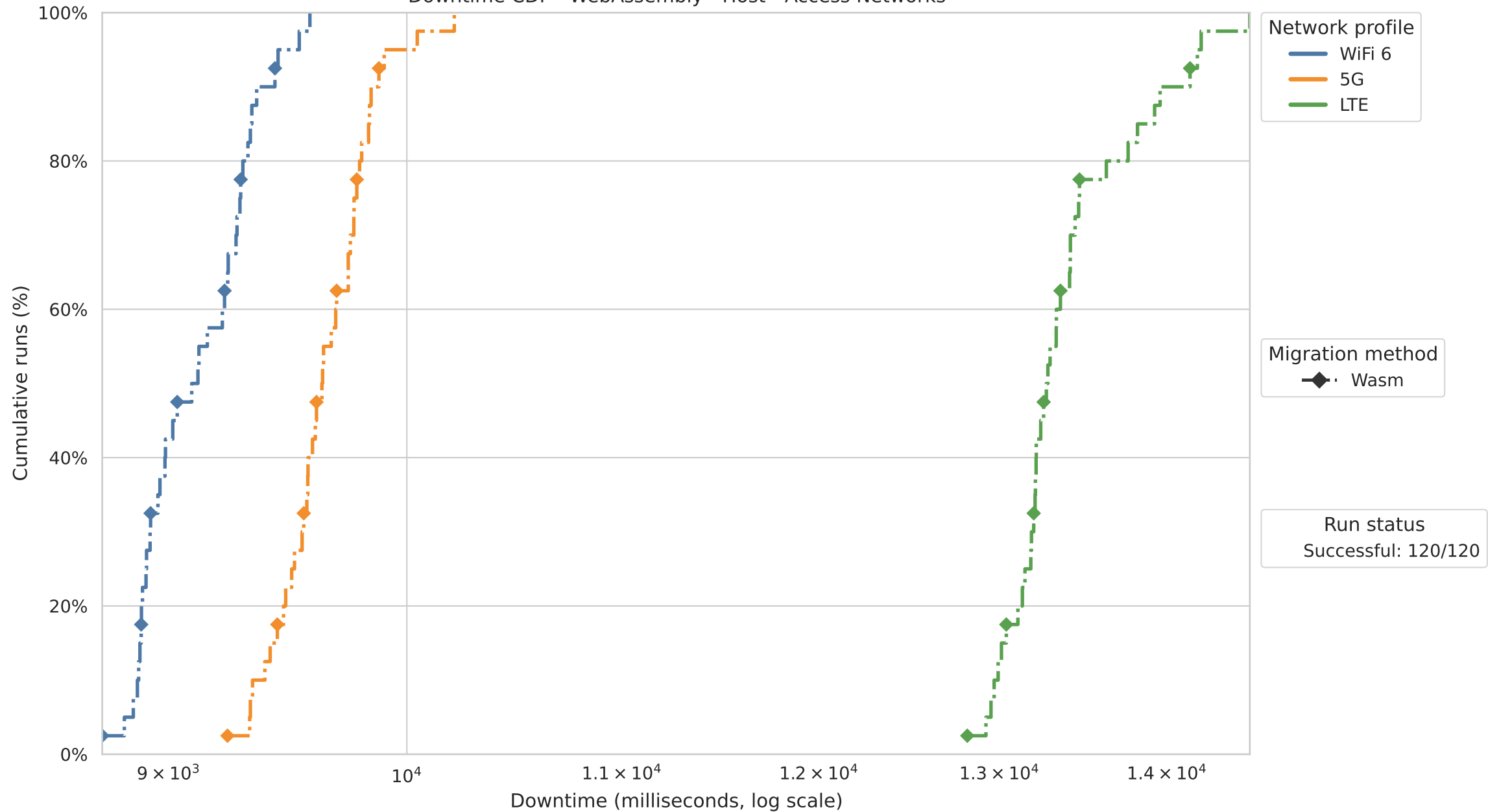
Downtime CDF - WebAssembly - Host - Access Networks
