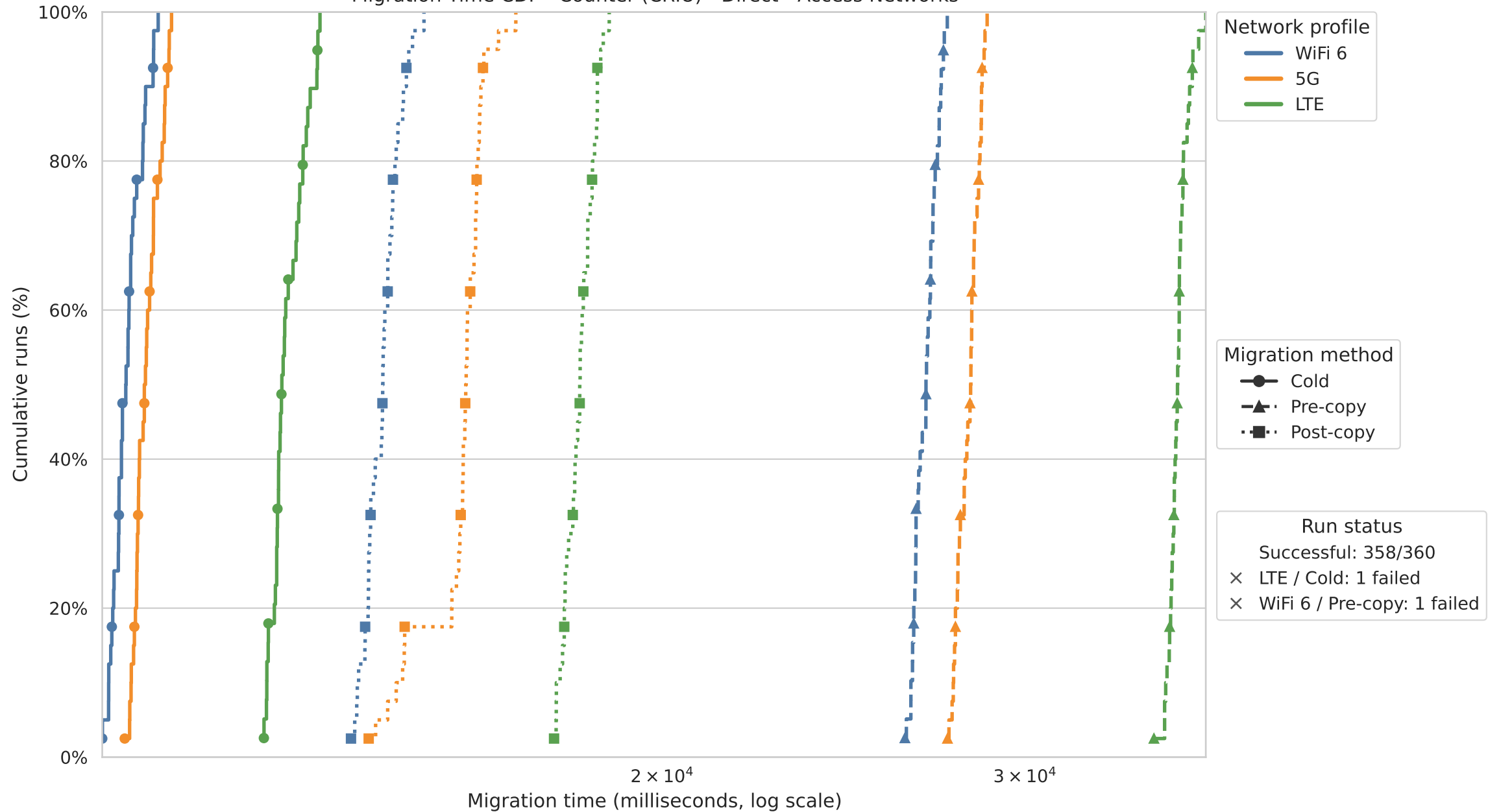
Migration Time CDF - Counter (CRIU) - Direct - Access Networks
