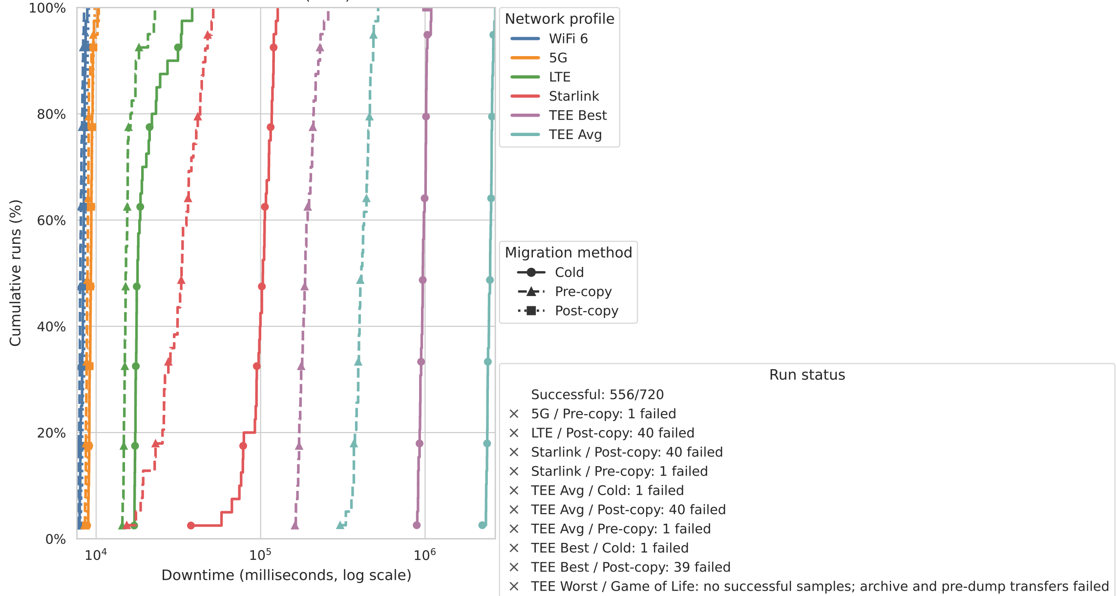
Downtime CDF - Game of Life (CRIU) - Host - All Profiles
