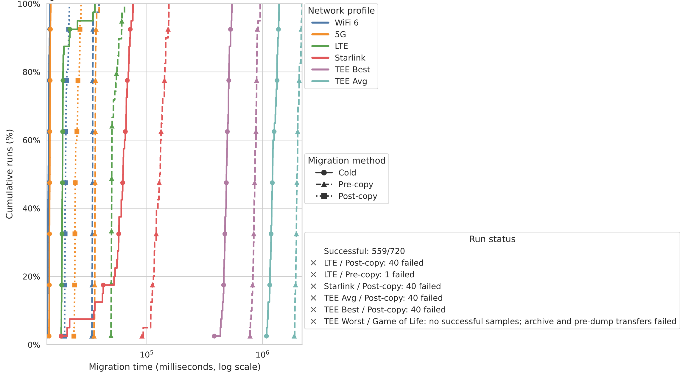
Migration Time CDF - Game of Life (CRIU) - Direct - All Profiles
