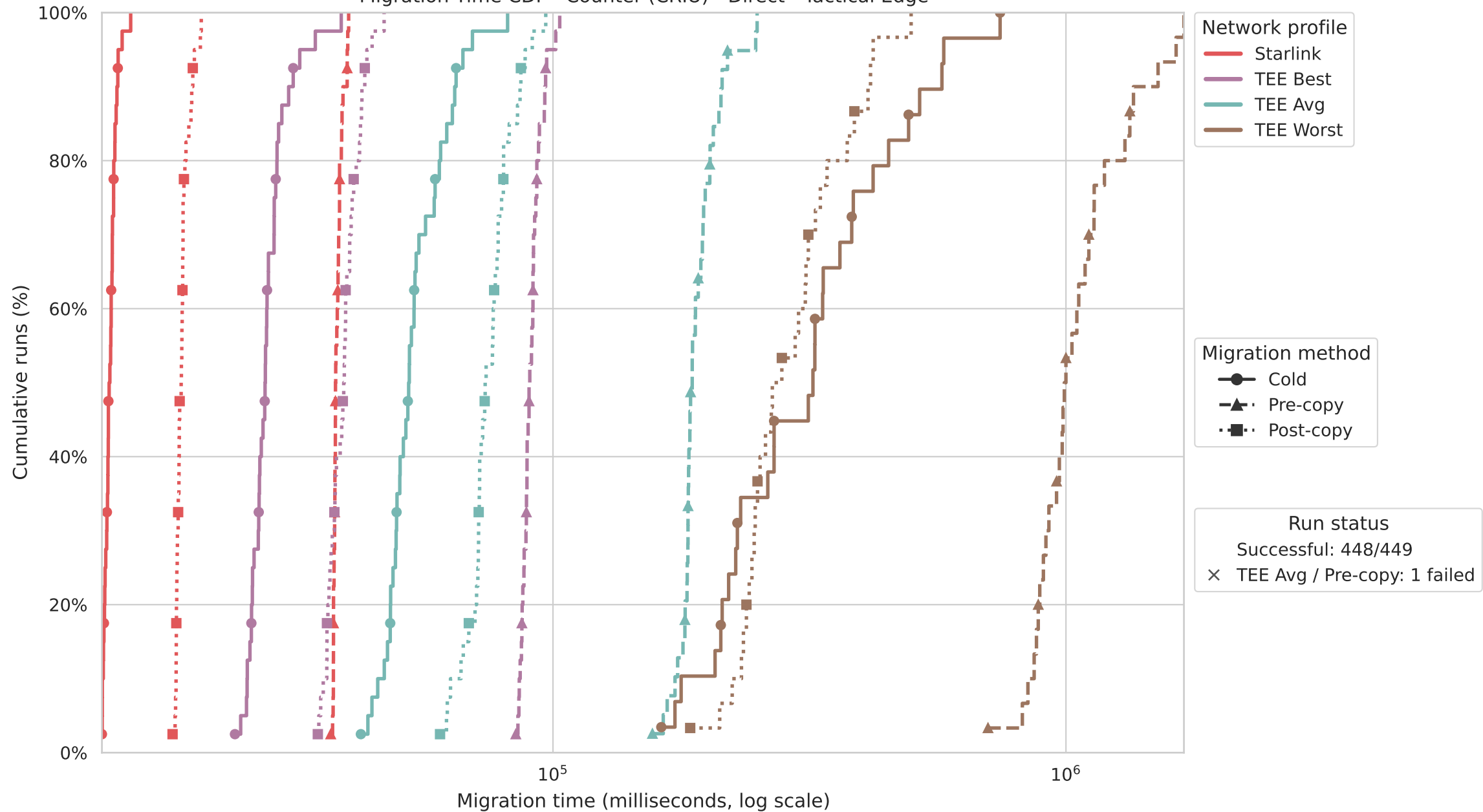
Migration Time CDF - Counter (CRIU) - Direct - Tactical Edge
