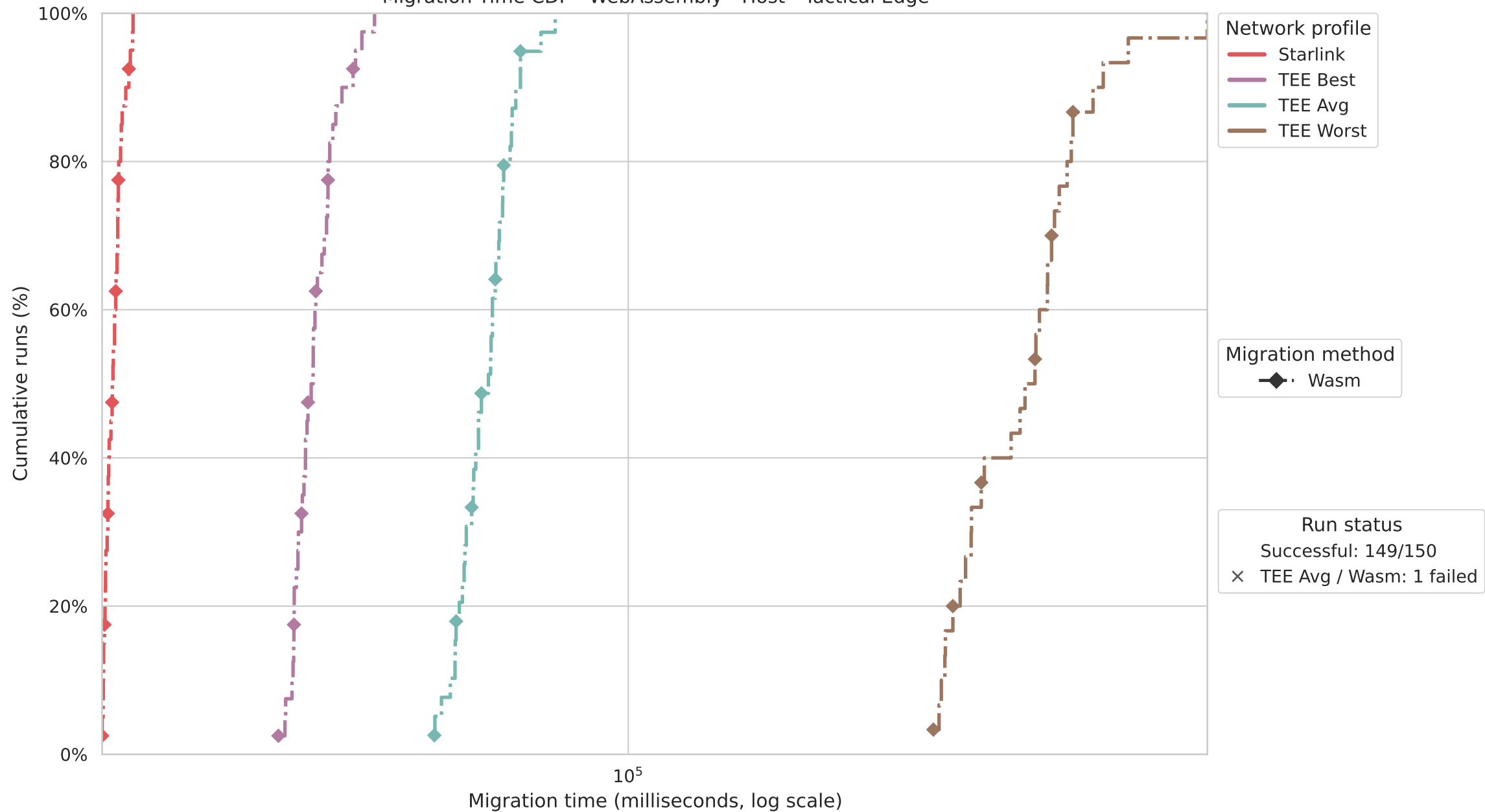
Migration Time CDF - WebAssembly - Host - Tactical Edge
