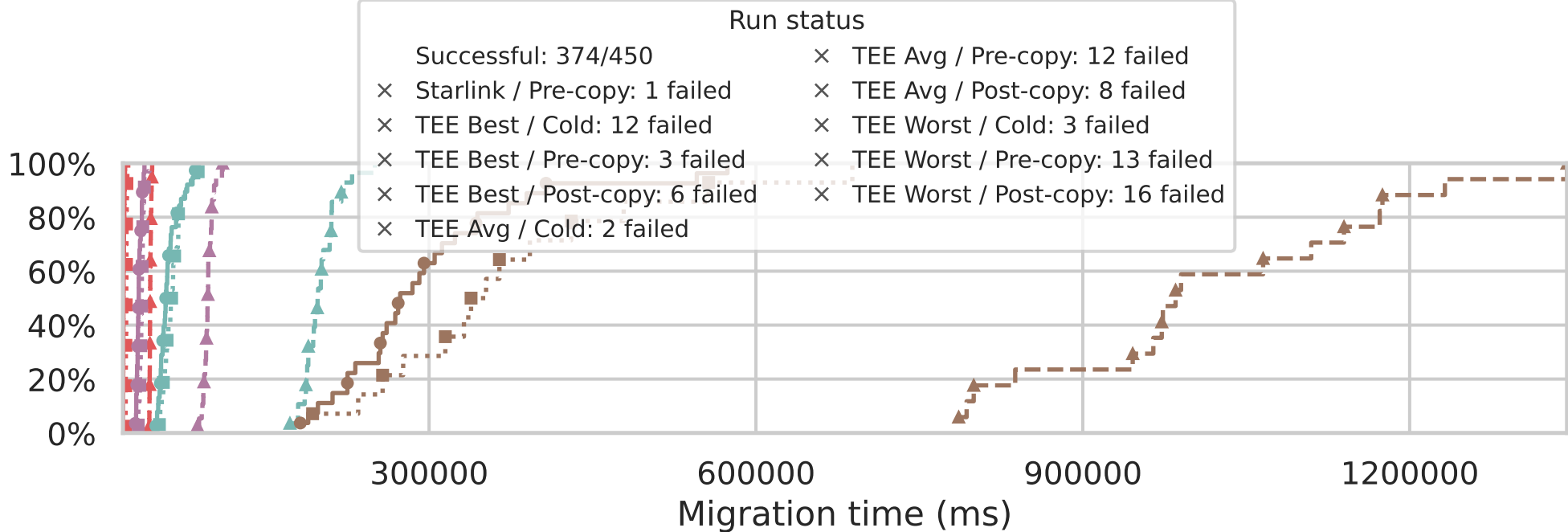
Cumulative runs (%)
