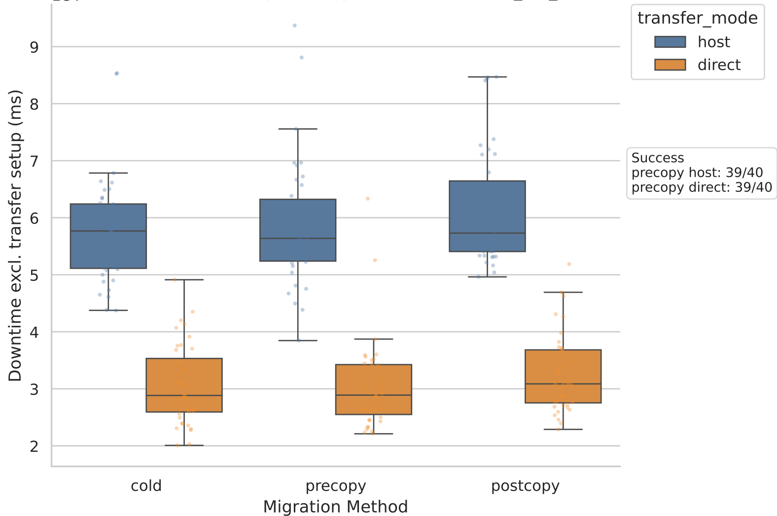
1e4 Migration Downtime by Strategy (Host vs Direct) - 6_tee_avg
