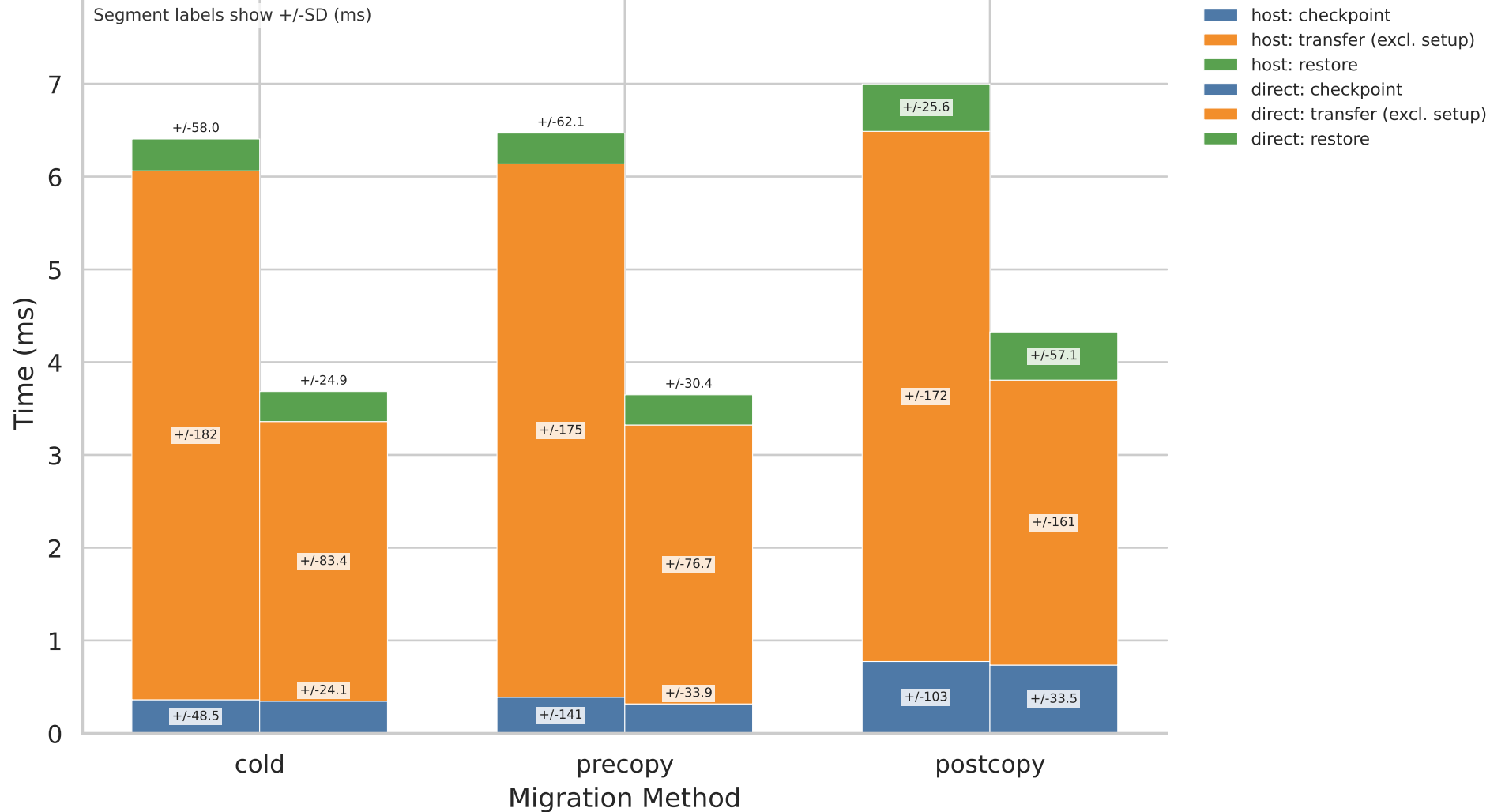
Migration Phase Breakdown (Mean) - 3_lte
