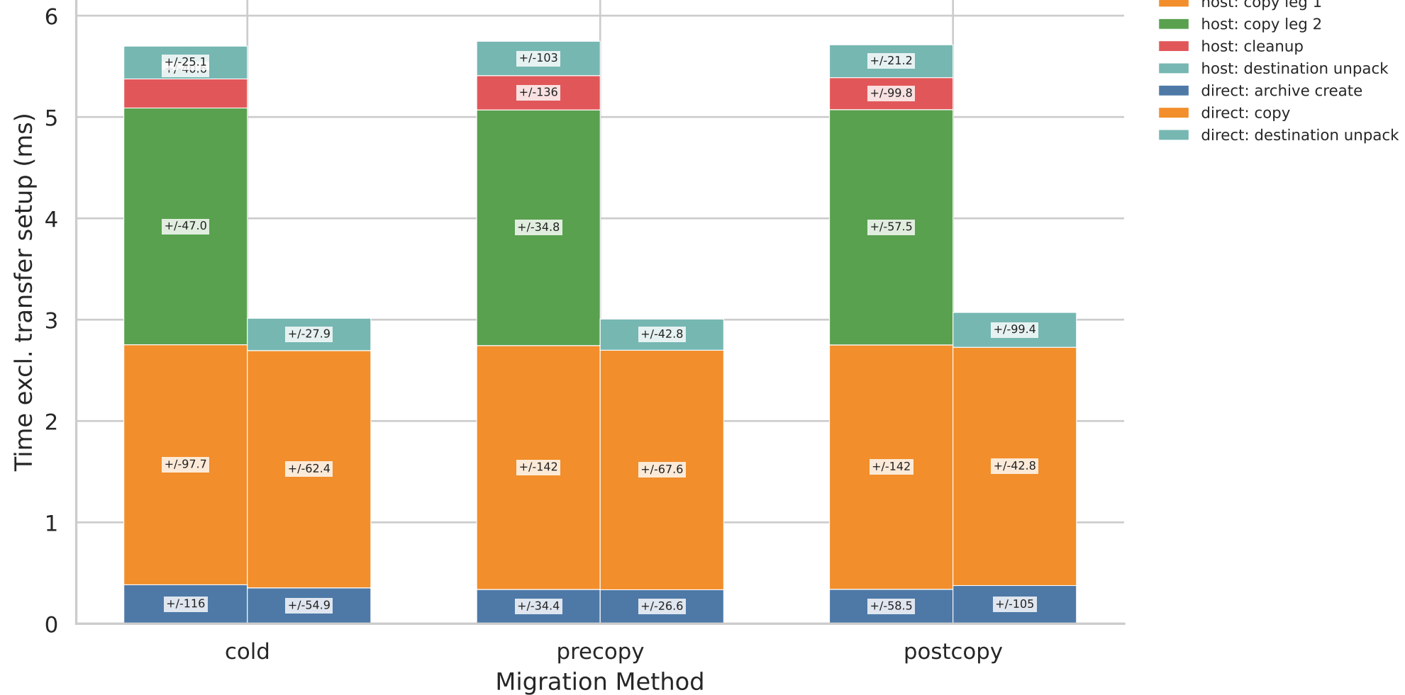
Transfer Phase Breakdown (Mean, setup excluded) - 3_lte
