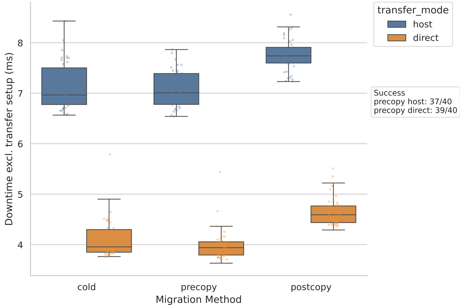
1e3 Migration Downtime by Strategy (Host vs Direct) - 4_starlink
