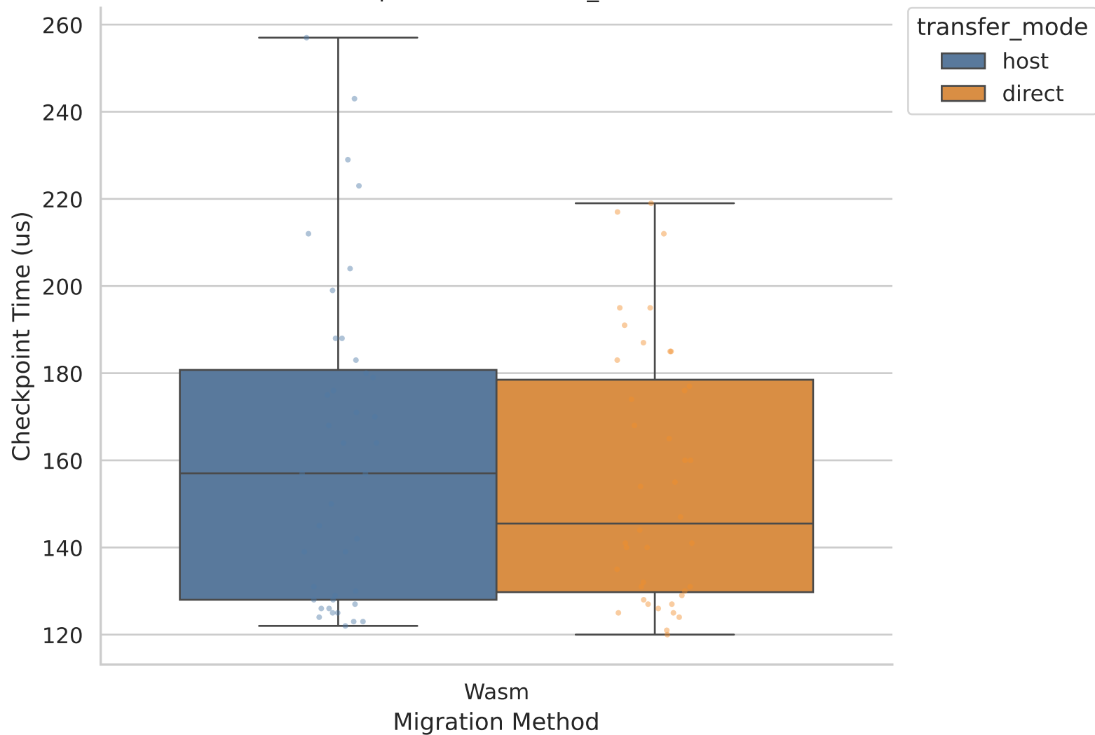
Checkpoint Duration - 4_starlink
