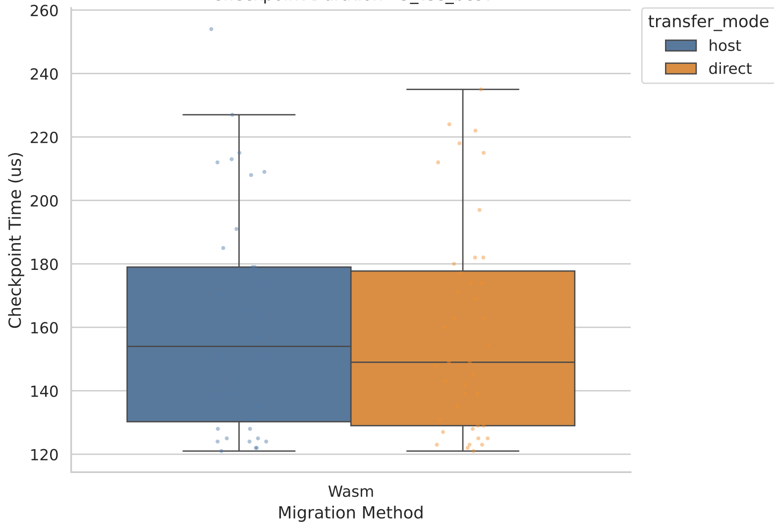
Checkpoint Duration - 5_tee_best
