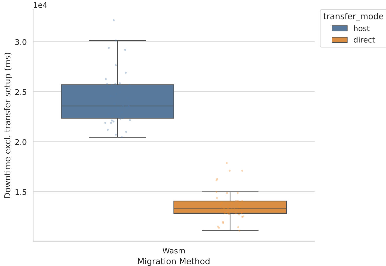
Migration Downtime by Strategy (Host vs Direct) - 5_tee_best
