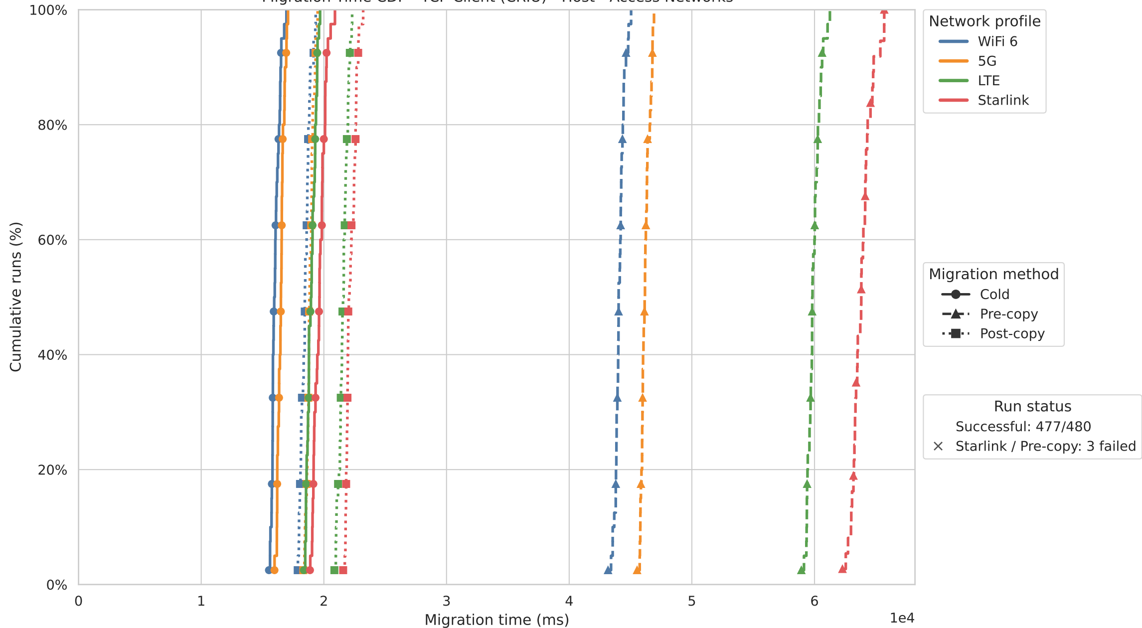
Migration Time CDF - TCP Client (CRIU) - Host - Access Networks
