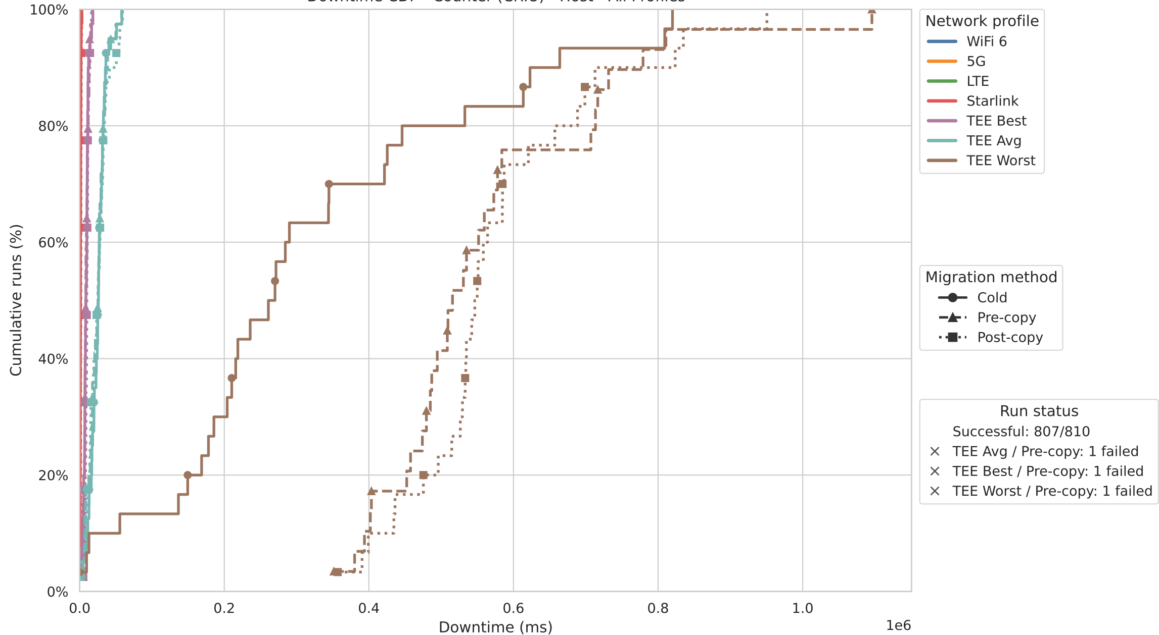
Downtime CDF - Counter (CRIU) - Host - All Profiles
